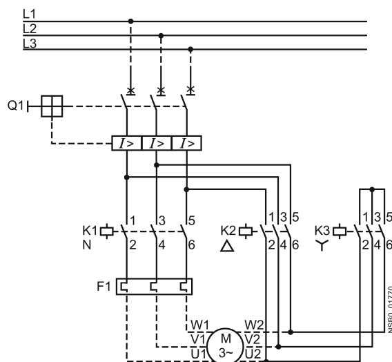
Circuit diagram main circuit for \text{Y}\Delta circuit
